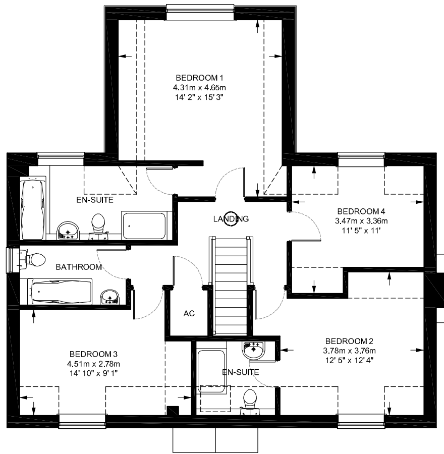
First Floor Plan Plot 4
