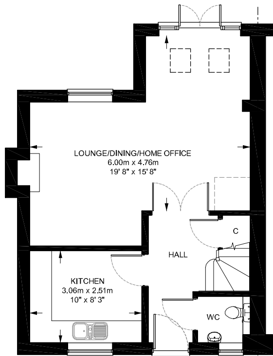
Ground Floor Plan Plot 3
