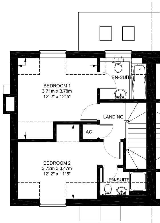
First Floor Plan Plot 3
