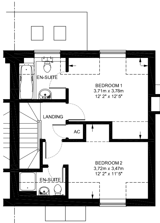
First Floor Plan Plot 2
