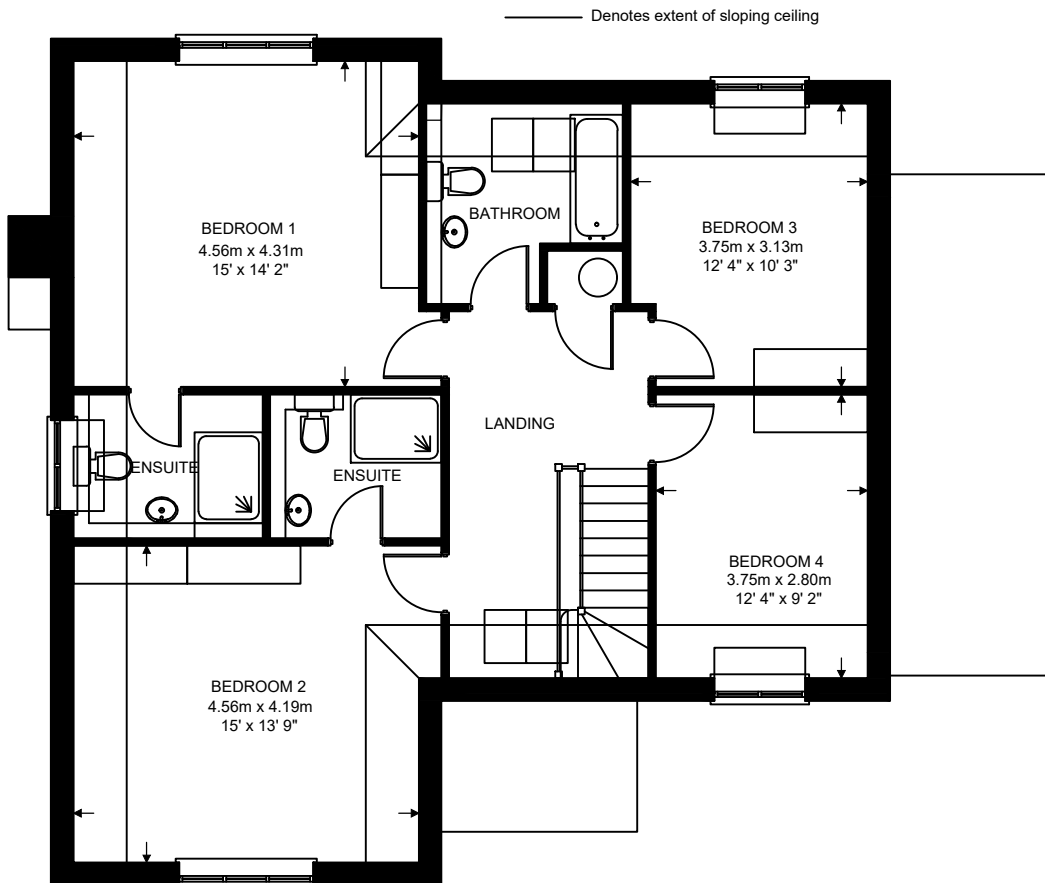
PLOT 1 FIRST FLOOR (PLOTS 2 AND 3 HANDED)
