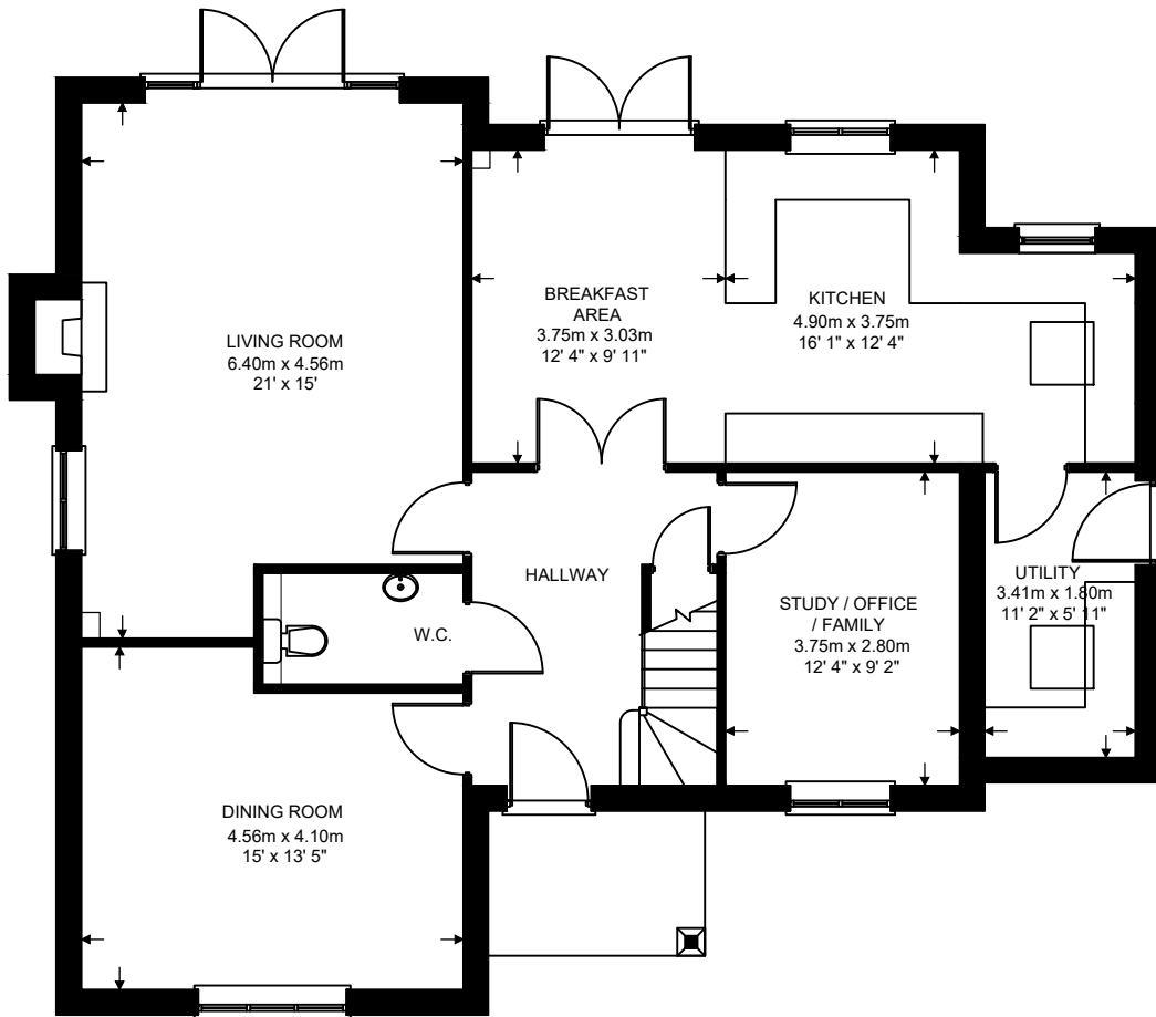
PLOT 1 GROUND FLOOR (PLOTS 2 AND 3 HANDED)
