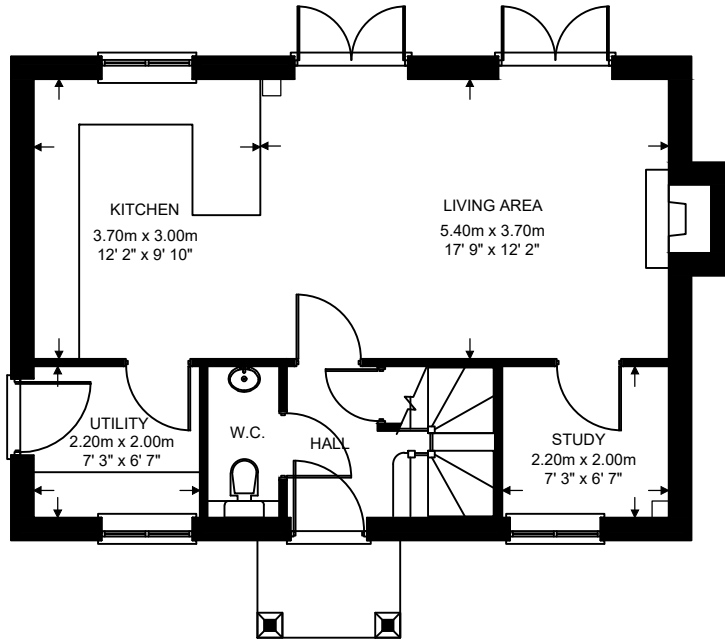
PLOT 4 GROUND FLOOR
