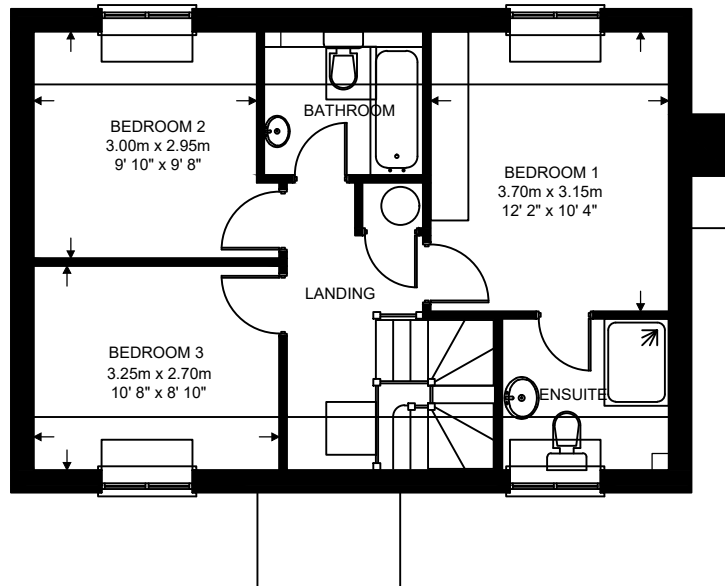
PLOT 4 FIRST FLOOR
